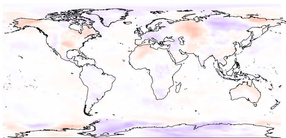
May temp2
