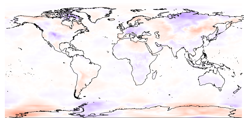
Jun temp2
