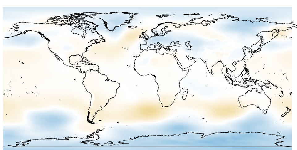
May slp
