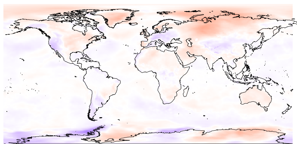
Apr temp2
