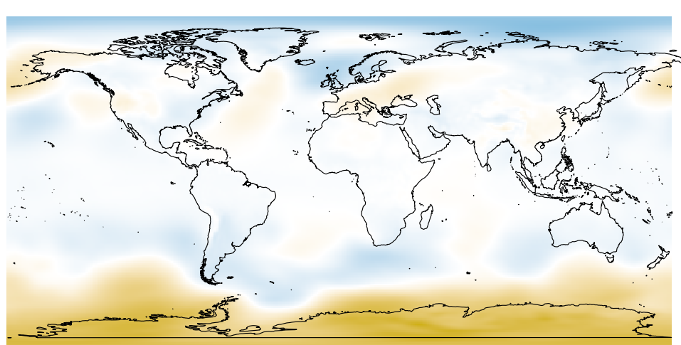
May slp
