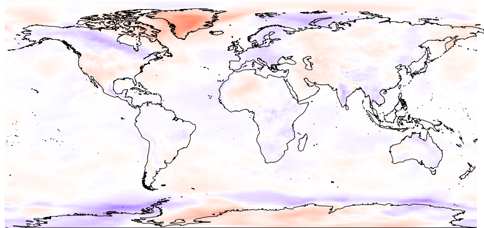
Apr temp2
