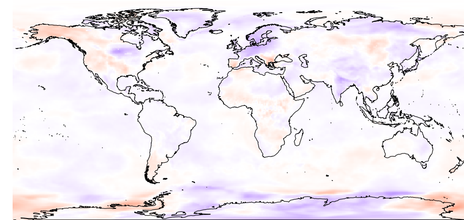
Jun temp2
