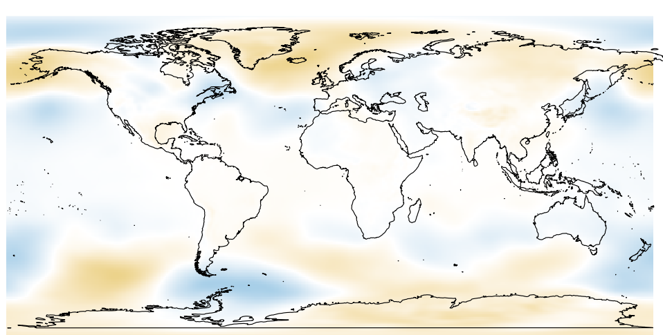
Apr slp
