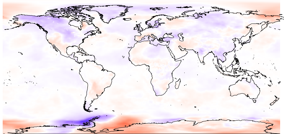
May temp2
