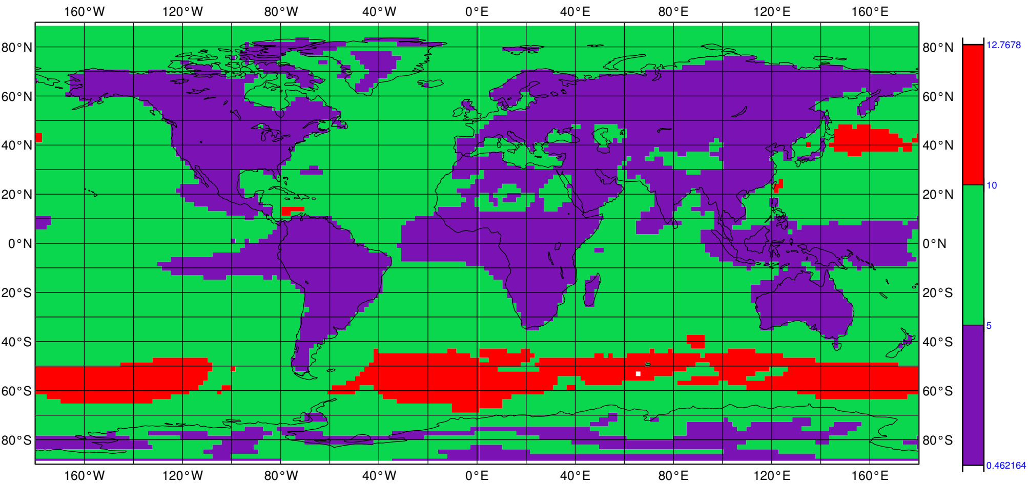
wind10 [m/s] 1855-07-01 08:52:00
