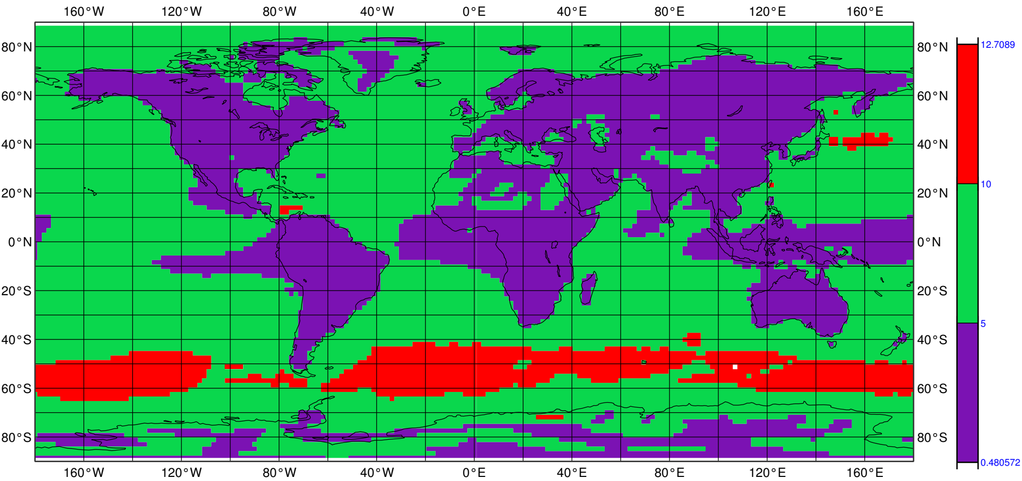
wind10 [m/s] 1866-07-01 08:52:00
