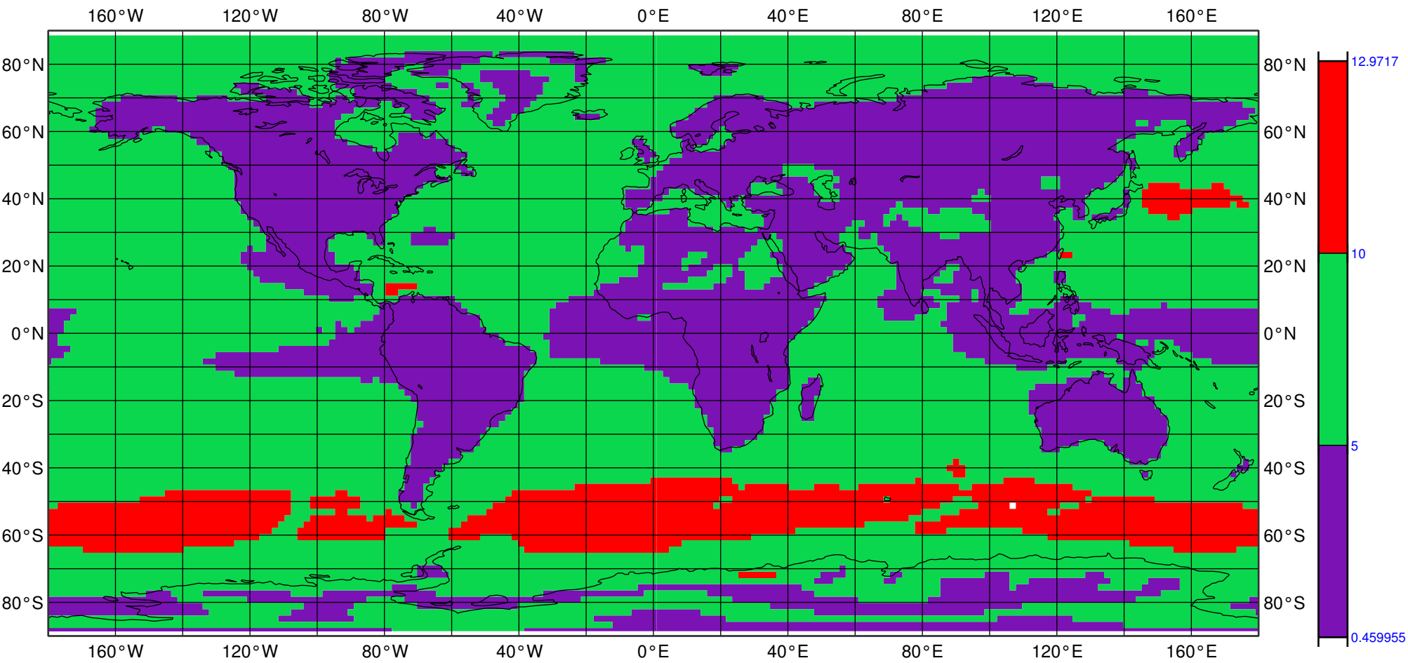
wind10 [m/s] 1887-07-01 08:52:00
